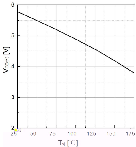
F 5. T V_{GE}(\text{th}) ( I_D = 1\text{ A} )
